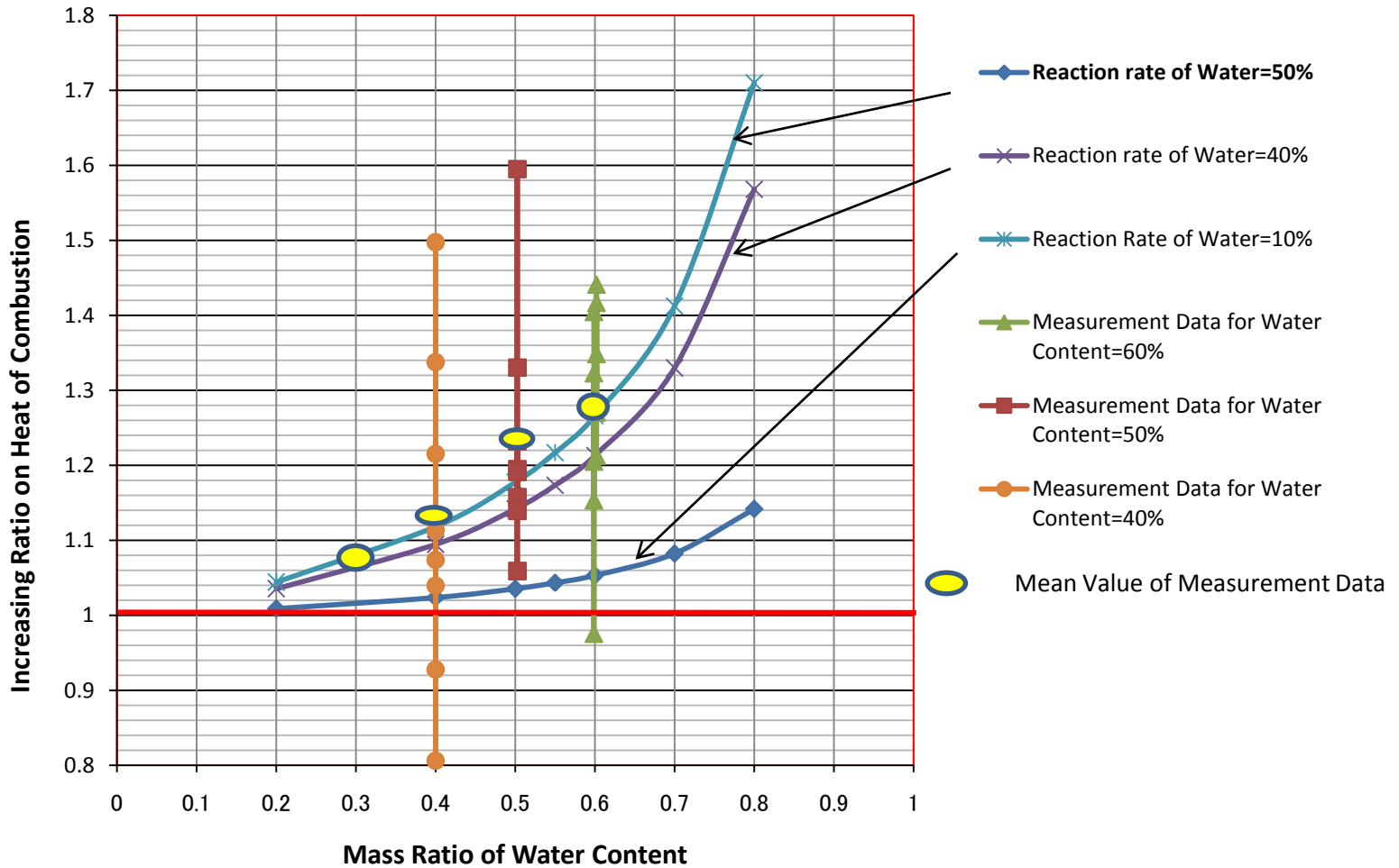
Fig.2 Measurement Results of Heat of Combustion for "Fukai Emulsion"
